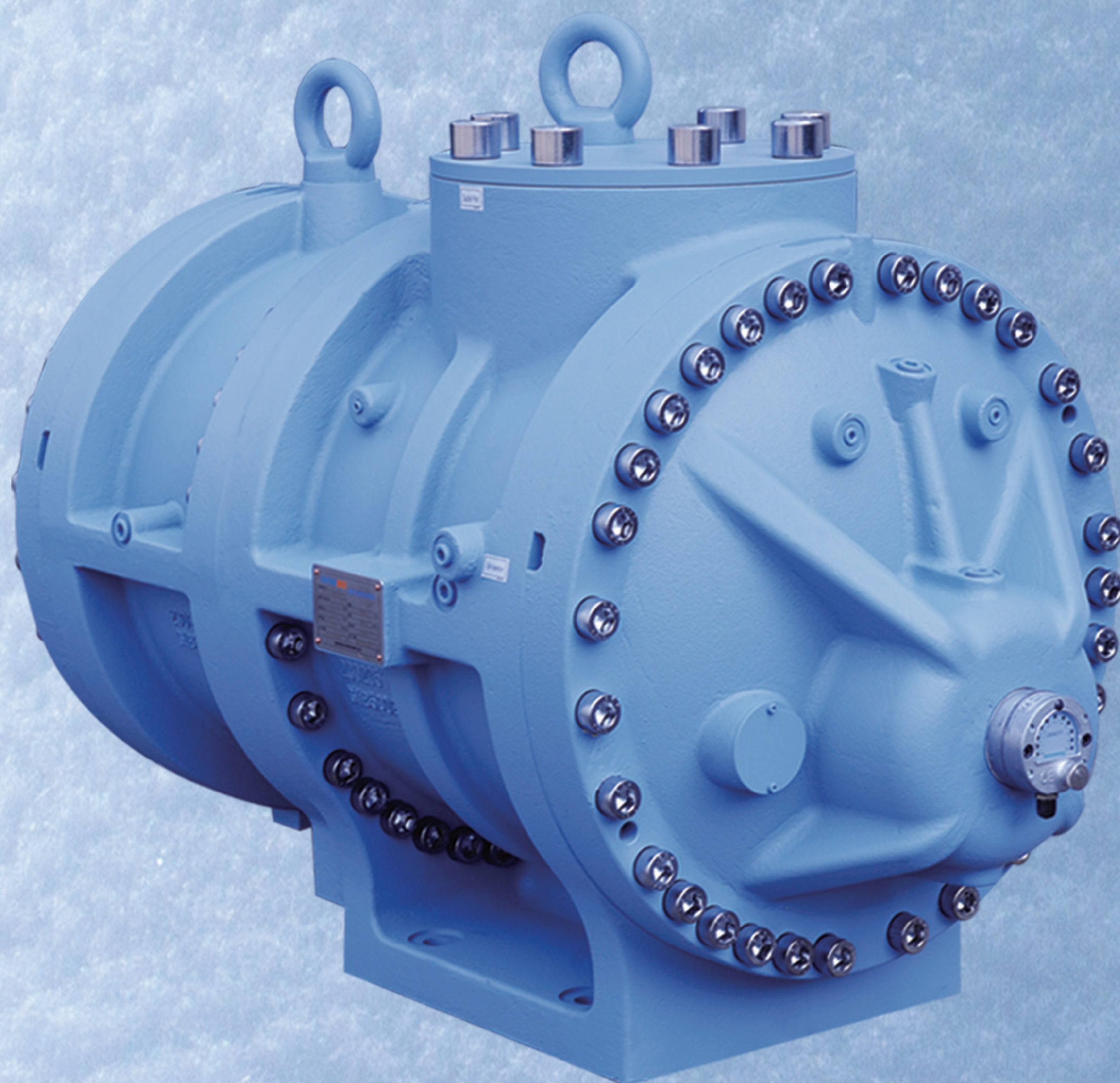
SRM - 18 Series SRH Open type screw compressor High pressure heat pump series
